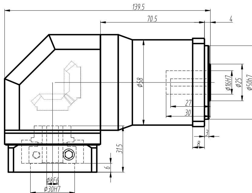
标准轴 Standard output shaft
